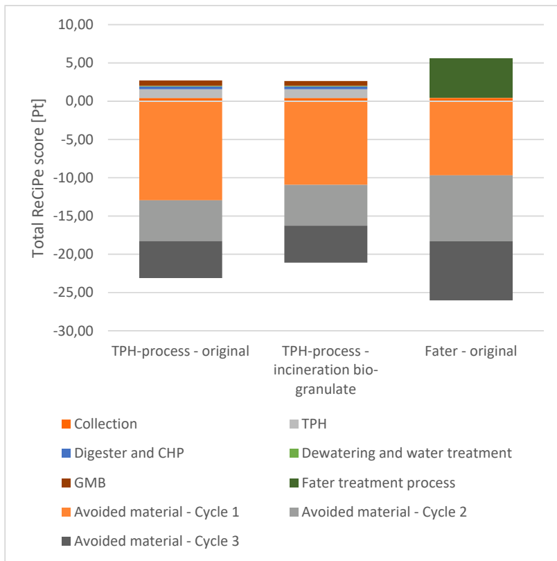
Figure 12 Results sensitivity analysis – waste incineration bio-granulate
