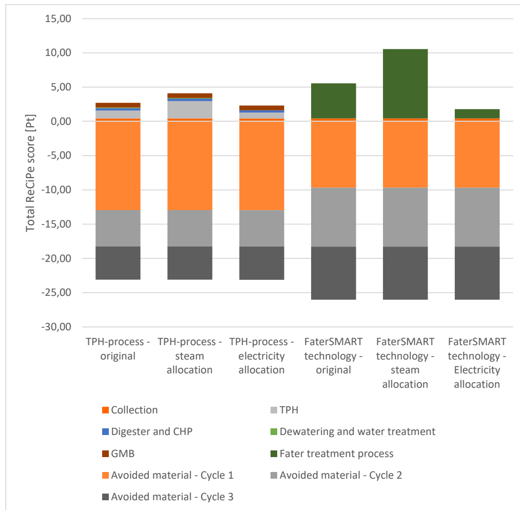
Figure 11 Sensitivity analysis steam and electricity allocation
